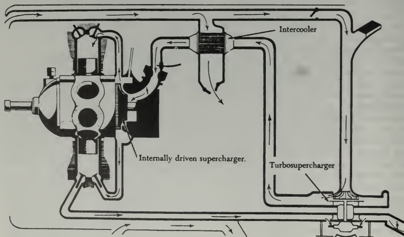
FIGURE 2-10. Induction system with turbosupercharger.
